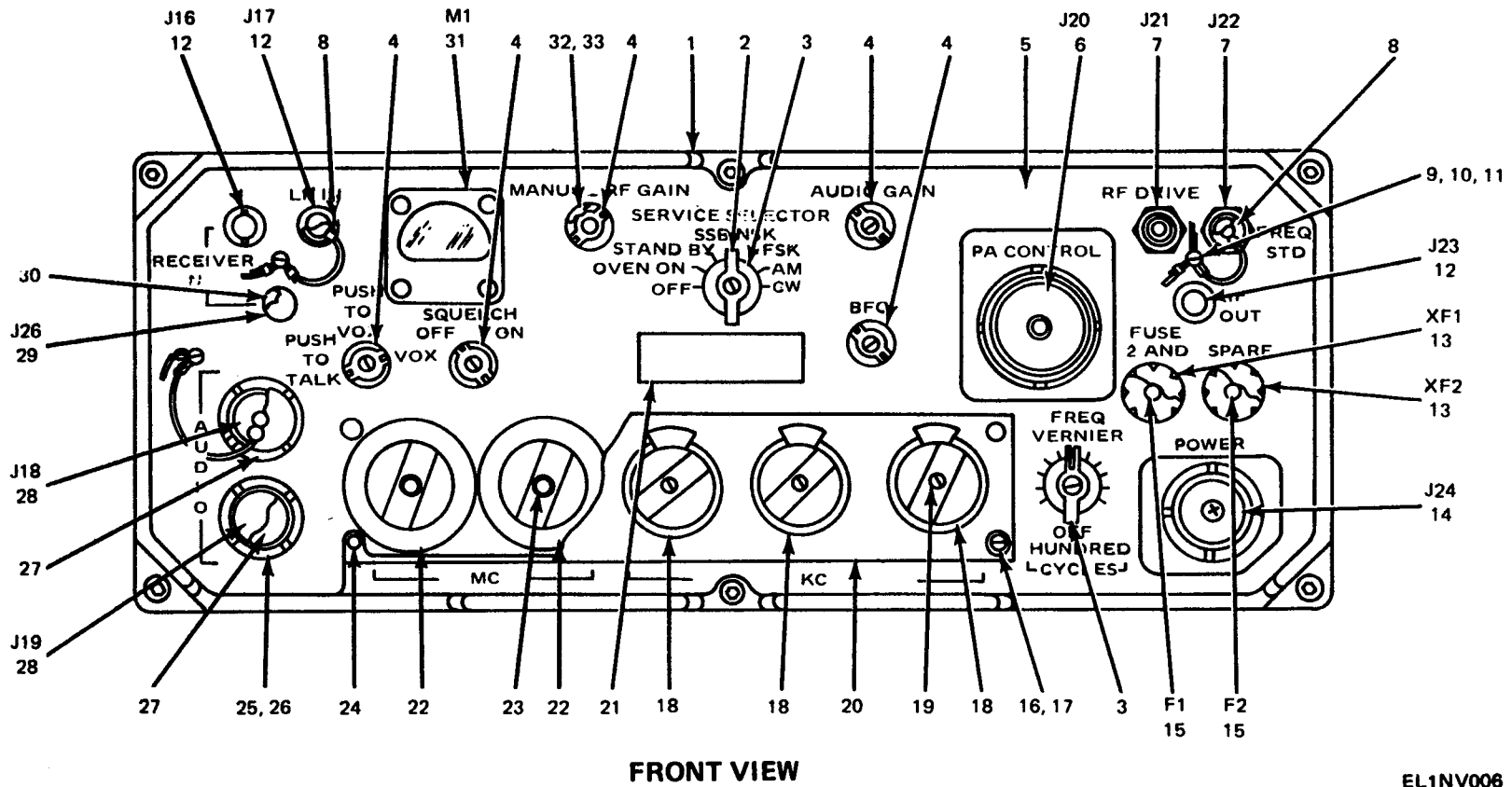
Figure 5. Chassis Assembly (1A1) (Sheet 1 of 5).
