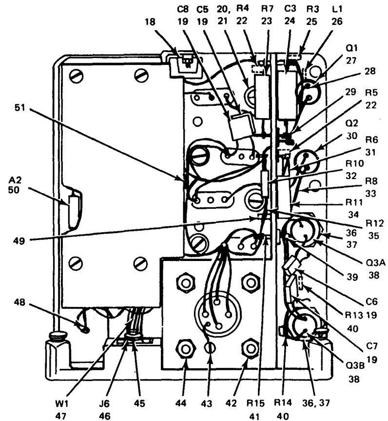
BACK VIEW
